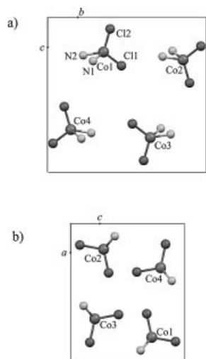
Figure 6. (a) Projection along a of the four Co II ions and their ligands in the unit cell for compound 1b . (b) Projection along b of the four Co II ions and their ligands in the unit cell for compound 1c .
