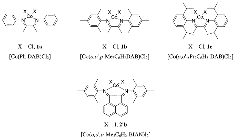
Scheme 1. Synthesized complexes.
